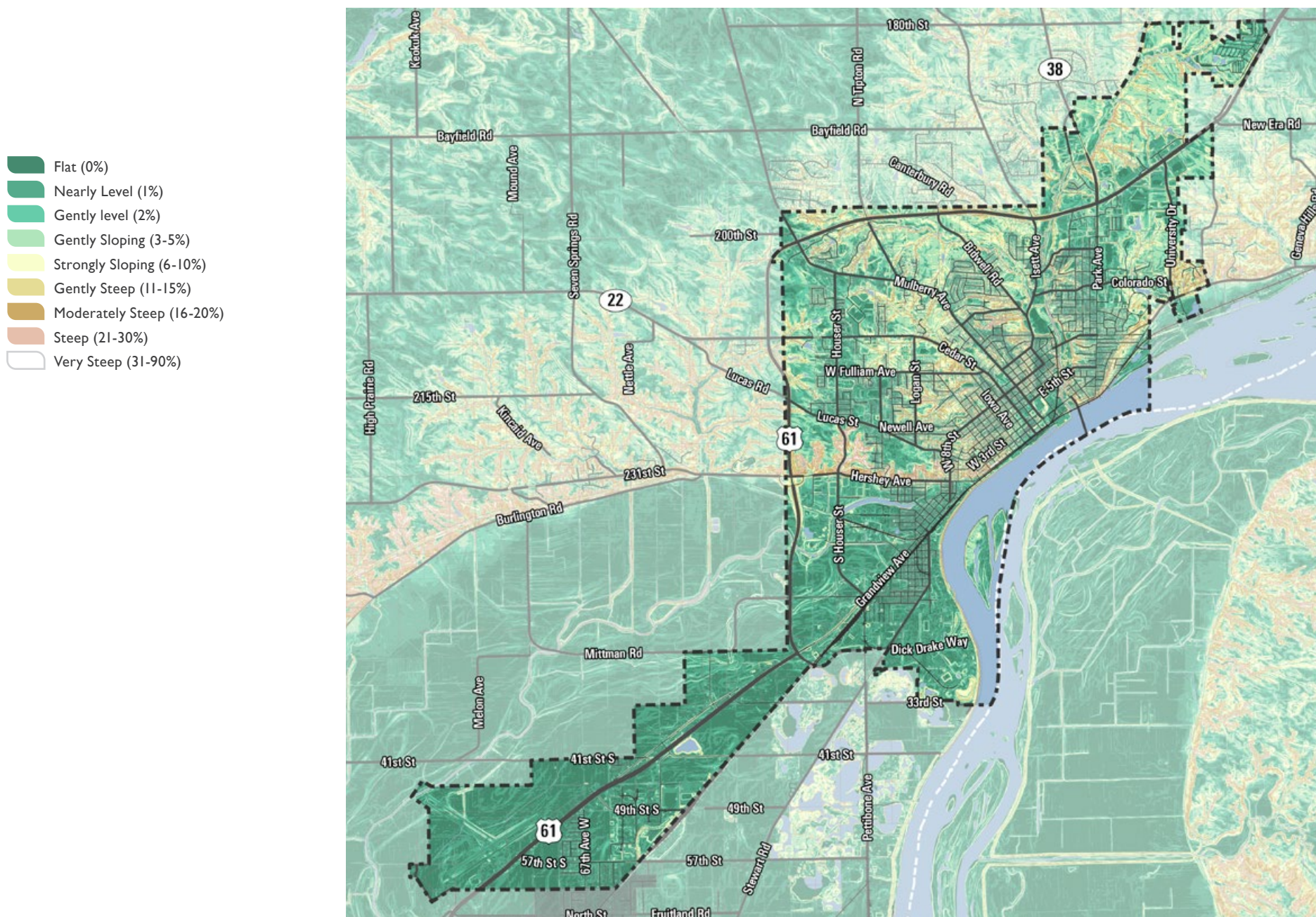
Figure A.3: Steep Slopes
